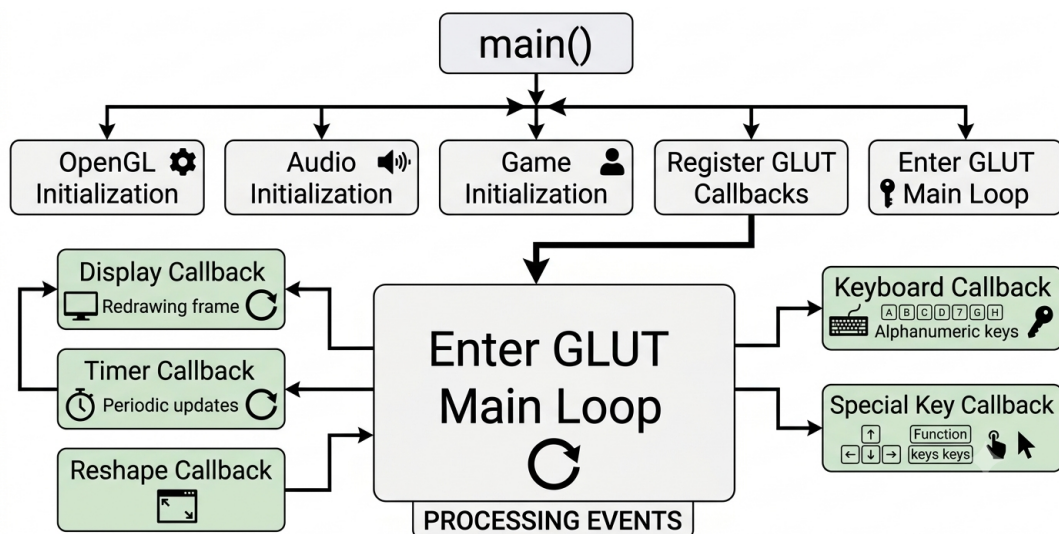
Figure 2.1: Application Initialization
